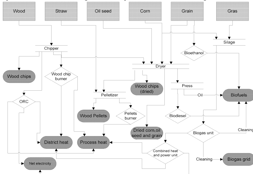
Fig. 2: Maximum Structure
